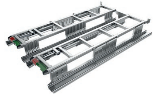
Lean Adapterpalette
